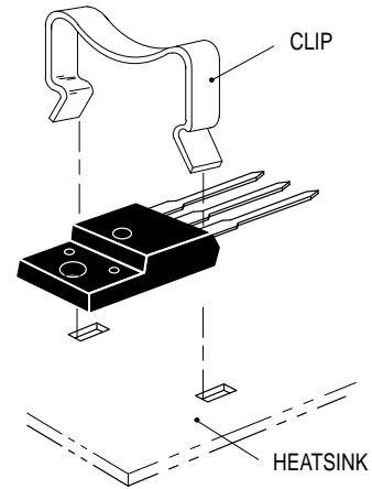
10b. Clip-Mounted
