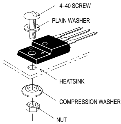
10a. Screw-Mounted
